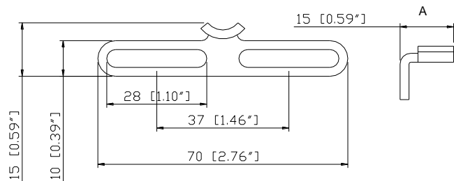
19068 Keeper W/Out Tab: A =15mm (0.590)
