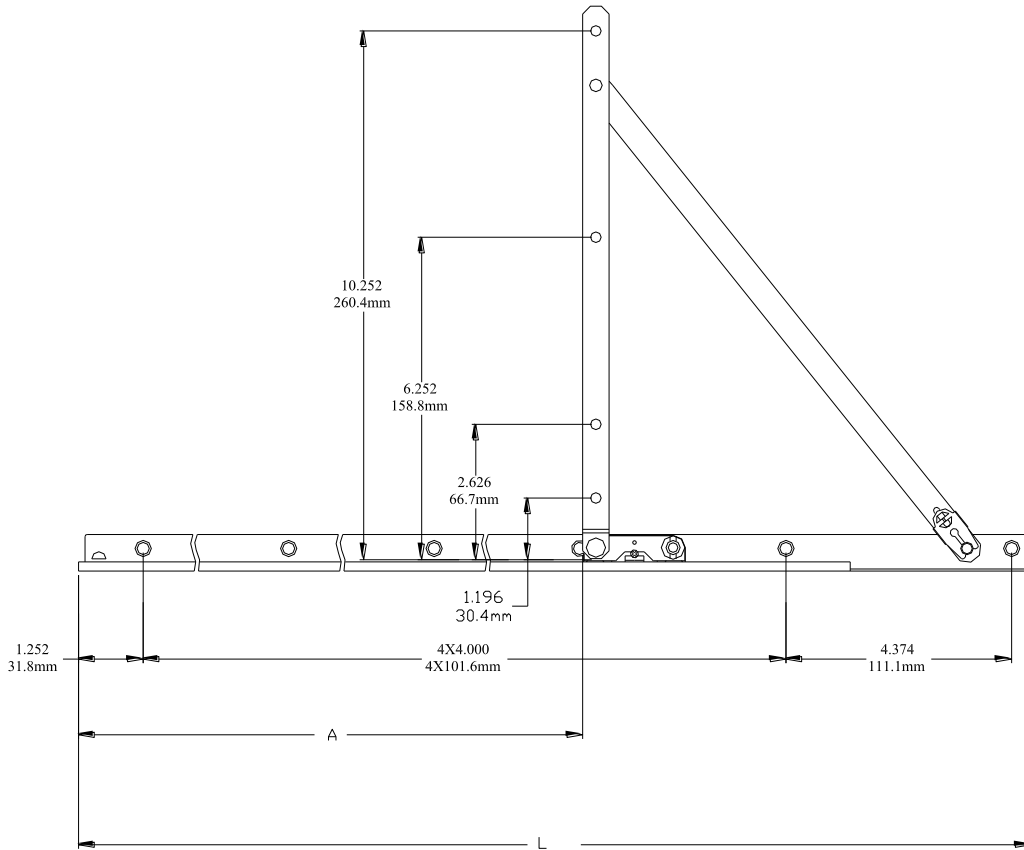
22" Standard Two Bar Hinge
