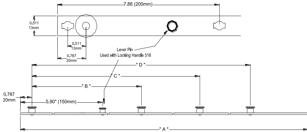
Tie Bar 198 Series
