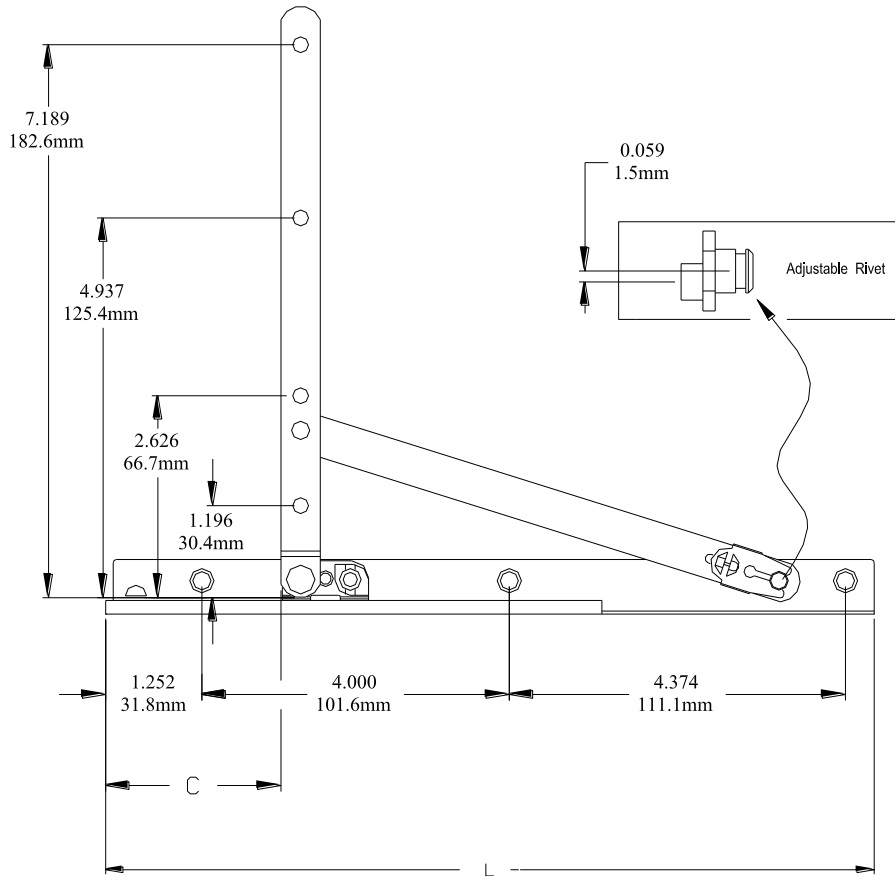
10" E Gress Two Bar Hinge
