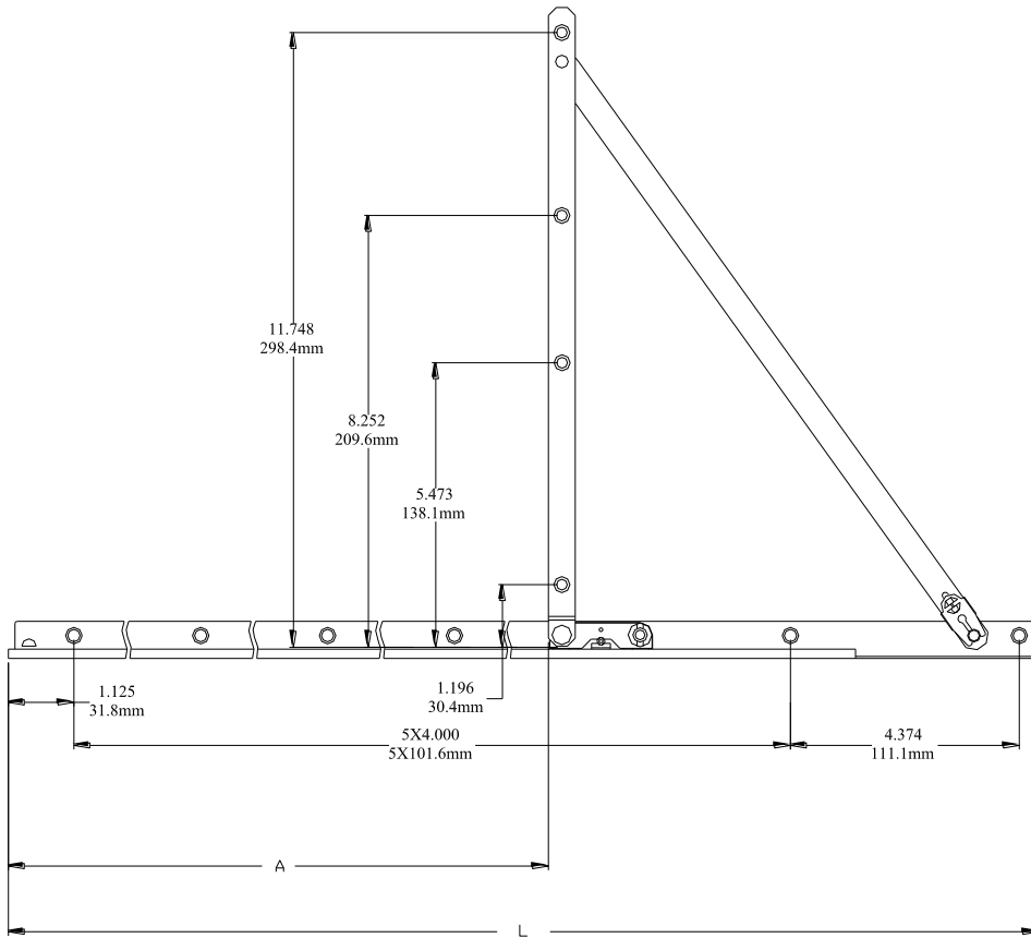
26" Standard Two Bar Hinge
