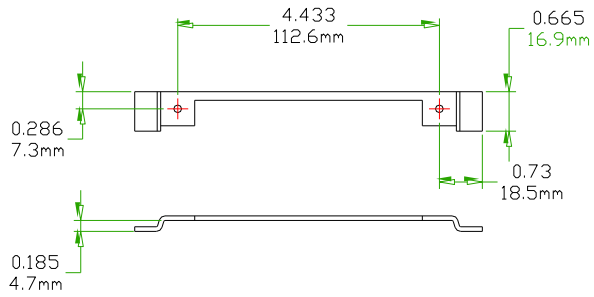
Track 190030 (Steel) / 70030 (Stainless Steel)
