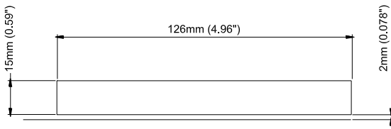
Frame Cut-out Details
