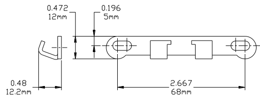
Sash Hook 19080 - Adjustable
