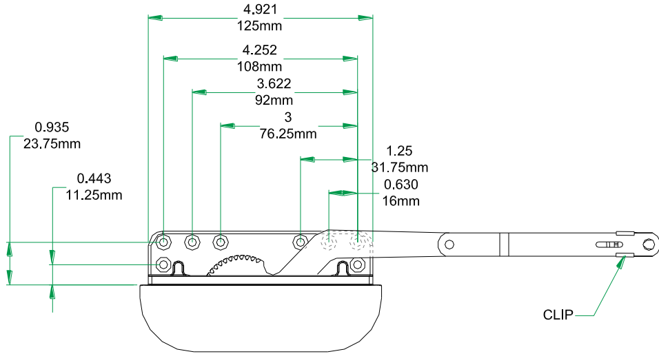
Left Hand Shown , Cover Closed
