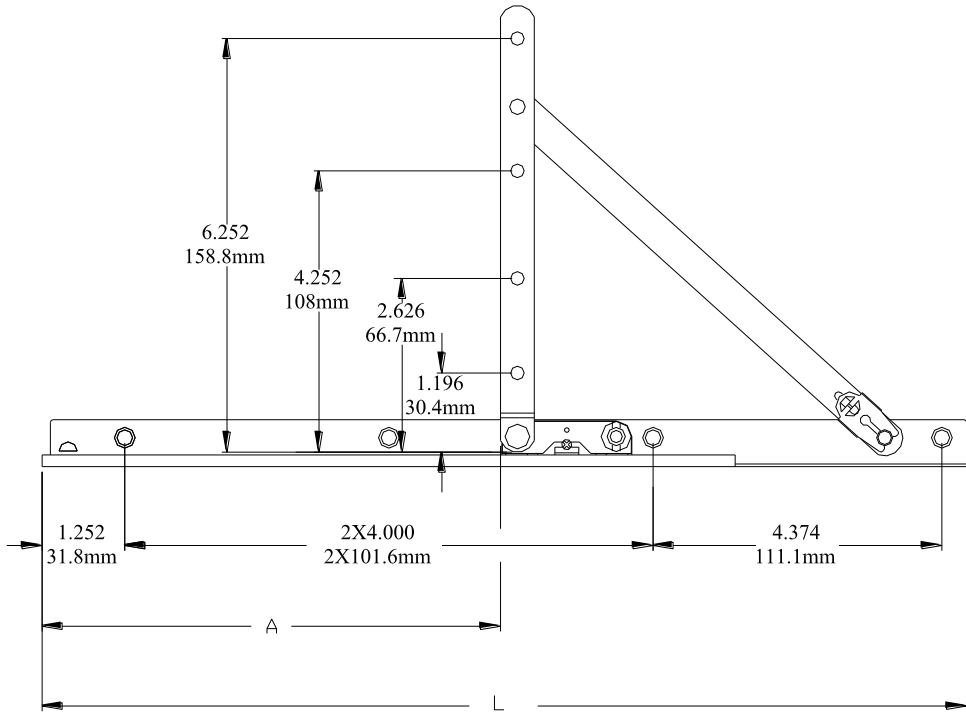
14" Standard Two Bar Hinge
