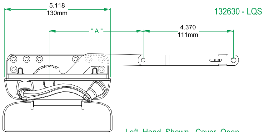
Left Hand Shown , Cover Open
