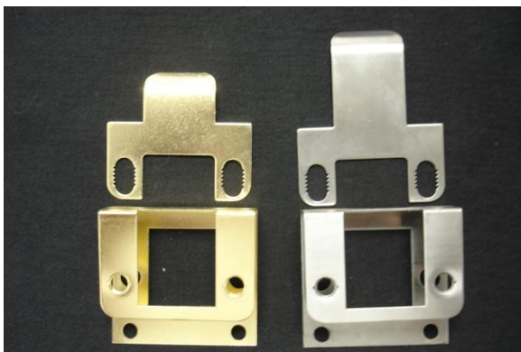
Single In- Swing Door Strike Plate
